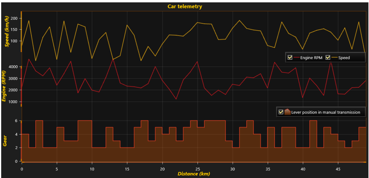
Figure 6-86. Position = SegmentBottomRight. AutoSpaceLegendBoxes = True.
