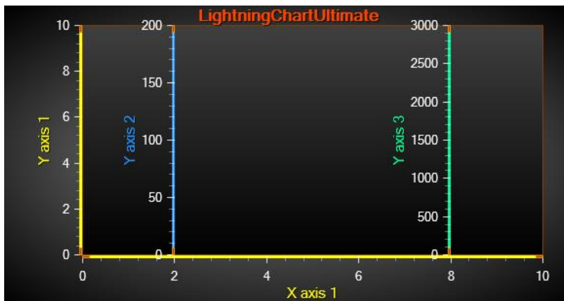
Figure 6-15. YAxisAutoPlacement = Off. Automatic axis placement is disabled, and Position and Alignment properties of each axis apply separately. First axis Position = 0, Second axis Position = 20 and Third axis position = 80.
