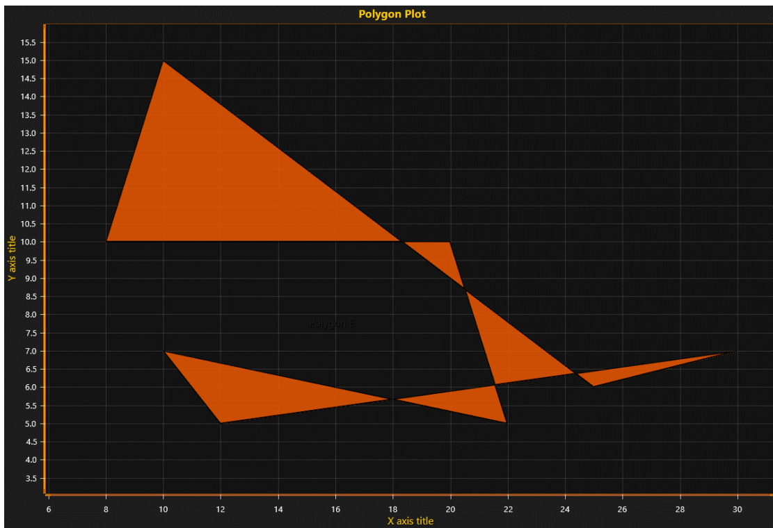
Figure 6-64. Polygon with intersecting path, with IntersectionsAllowed = True .
