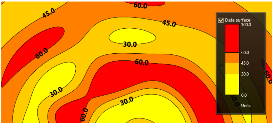
Figure 6-73. The properties of ContourLineLabels and the result
